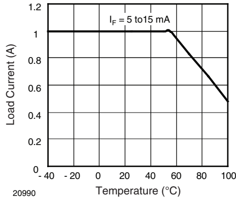
Figure 1. I_{LOAD} vs. Temperature
