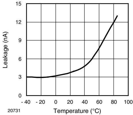
20731 Figure 4. Typical Leakage vs. Temperature ( V_{Load} = 60 V )
