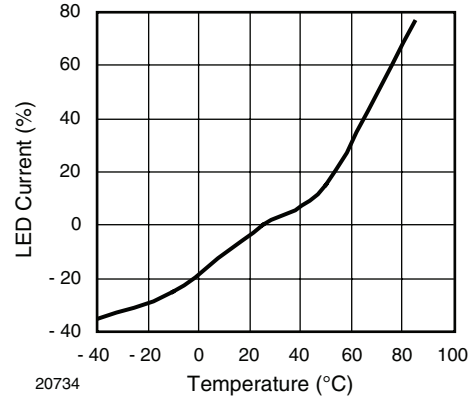
20734 Figure 7. I_F For Switch Operation vs. Temperature (Normalized to 25 °C, Load Current = 1 A)
